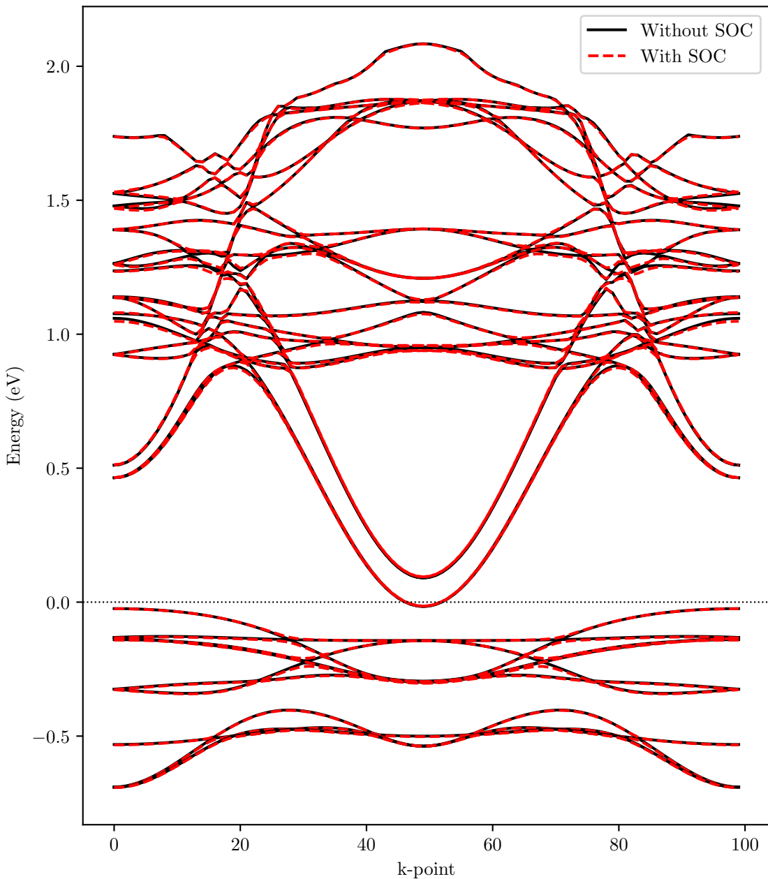
Band structure with and without SOC
